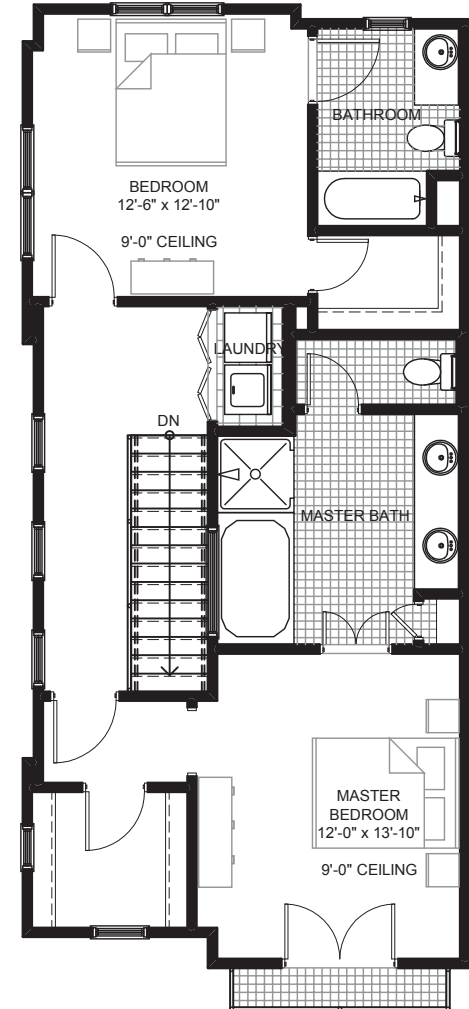
PLAN 3 TOWNHOME A1- 3RD FLOOR 1/4"=1'-0" A4.01 UNIT 101 809 HSF
